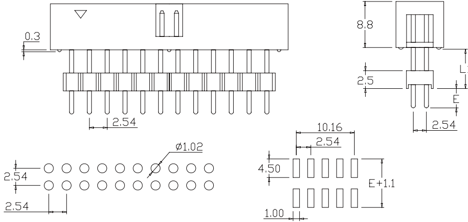
Recommended PCB Layout (PCB TOLERANCE±0.05)
